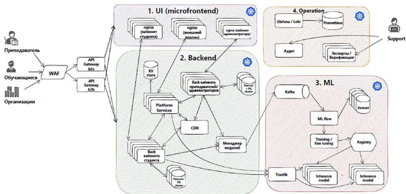
Архитектура DeepTalk
